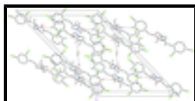
Fig. 2. The crystal packing of the title compound (I) with hydrogen bonds shown as dashed lines. H atoms not involved in the intermolecular interactions have been omitted for clarity.
